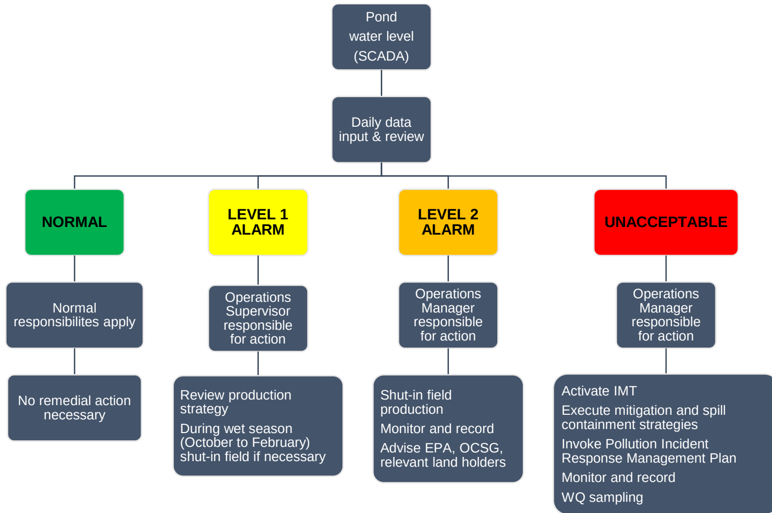
Figure 10.1 - Pond level principal response flowchart
