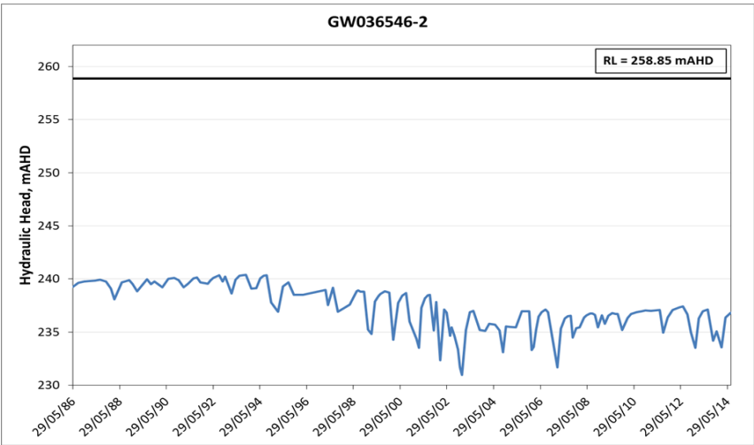
Figure A-18 Hydrograph for monitoring bore GW036546-2 (Namoi Alluvium)
