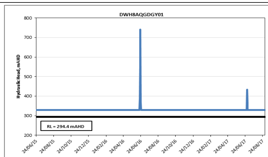
Figure A-45 Hydrograph for monitoring bore DWH8AQGDGY01 (Digby Fm)
