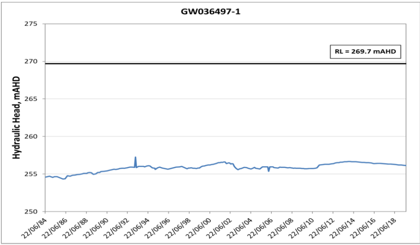
Figure A-20 Hydrograph for monitoring bore GW036497-1 (Namoi Alluvium)
