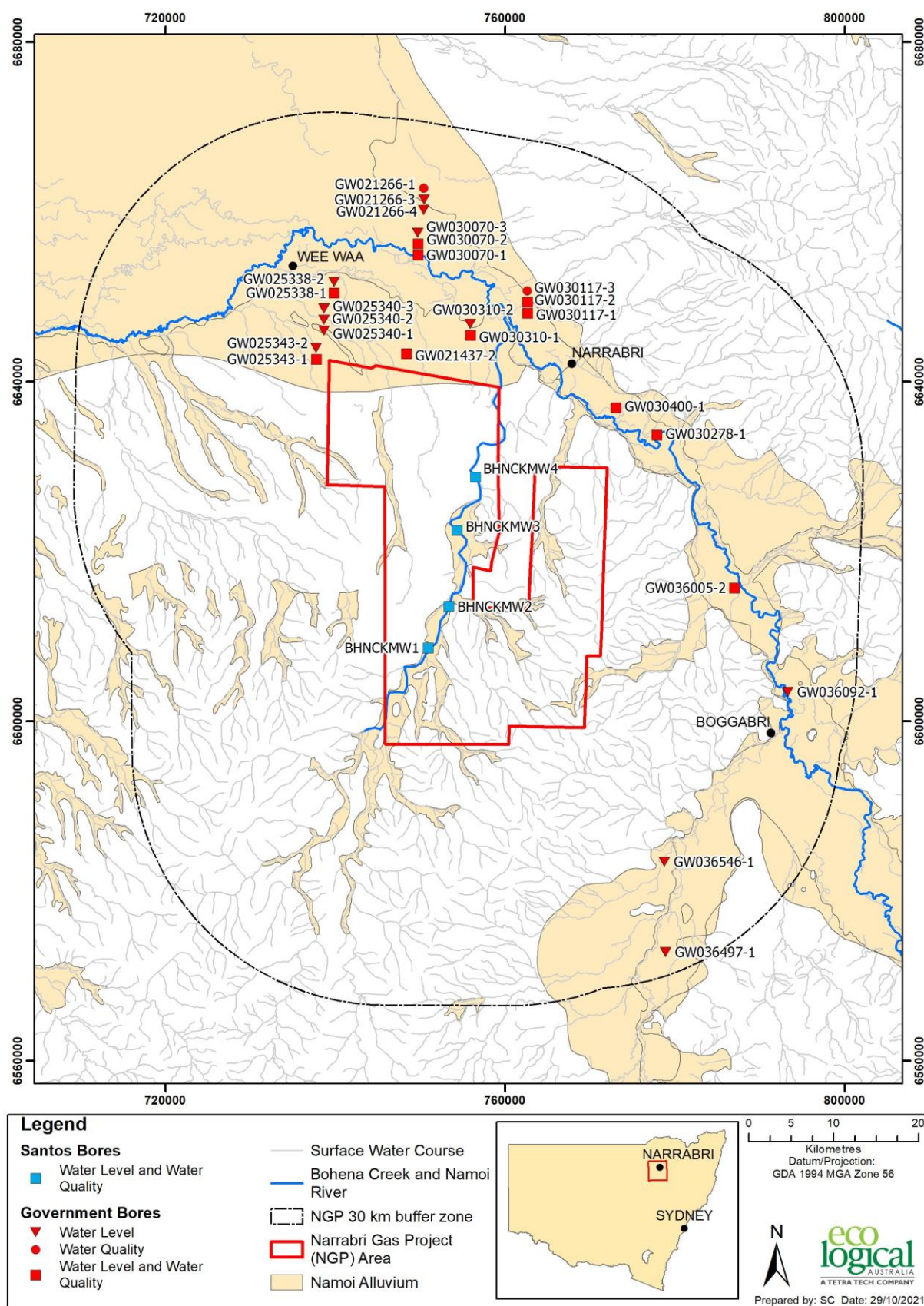
Figure 4.2 – Nominated alluvial aquifer groundwater monitoring points
