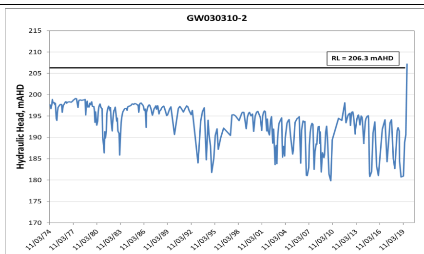
Figure A-21 Hydrograph for monitoring bore GW030310-2 (Namoi Alluvium)
