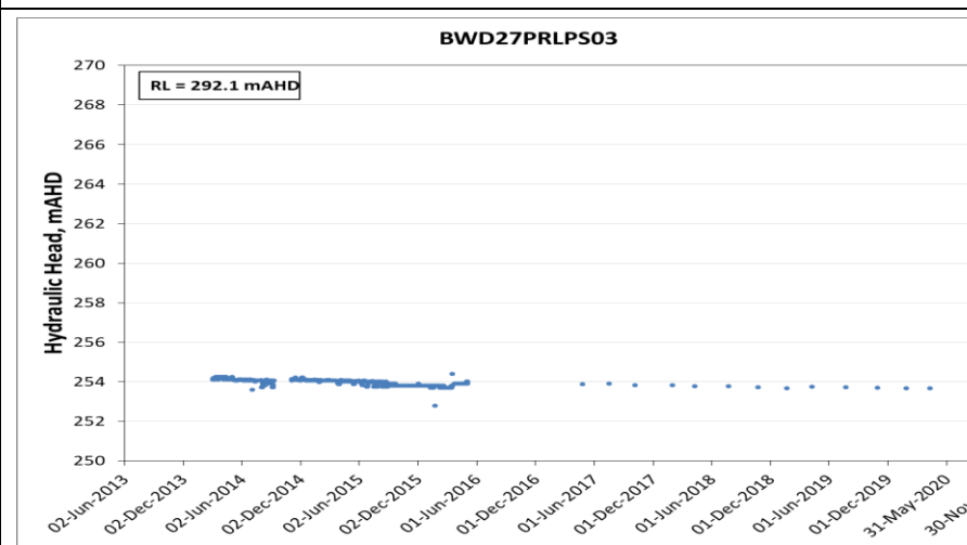
Figure A-32 Hydrograph for monitoring bore BWD27PRLPS03 (Pilliga Sandstone)
